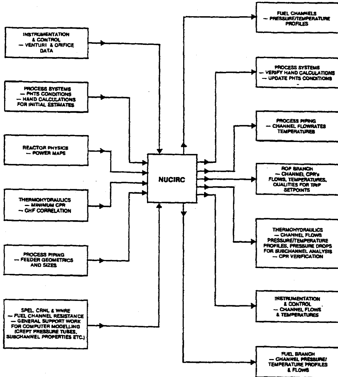
Figure 7.4 NUCIRC interaction
